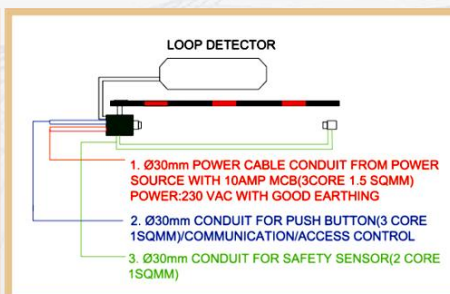
ELECTRICAL PROVISIONS
