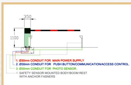
CIVIL PROVISIONS
